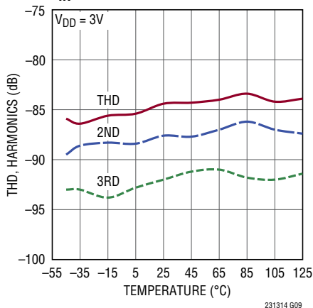
THD, Harmonics vs Temperature, f_{IN} = 497\text{kHz}
