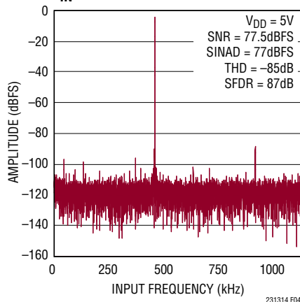
16k Point FFT, f_S = 2.5\text{Mpsps} f_{IN} = 497\text{kHz}
