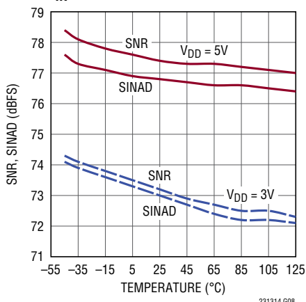
SNR, SINAD vs Temperature, f_{IN} = 497\text{kHz}
